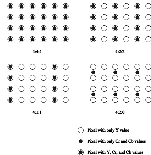
Fig. 5.6: Chroma subsampling
