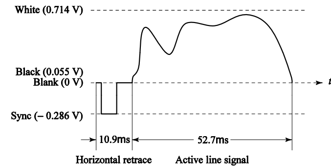
Fig. 5.3 Electronic signal for one NTSC scan line.
