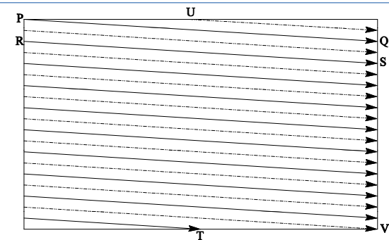
Fig. 5.1: Interlaced raster scan
