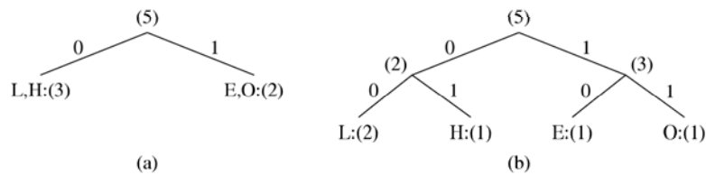
Fig. 7.4 Another coding tree for HELLO by Shannon-Fano.
