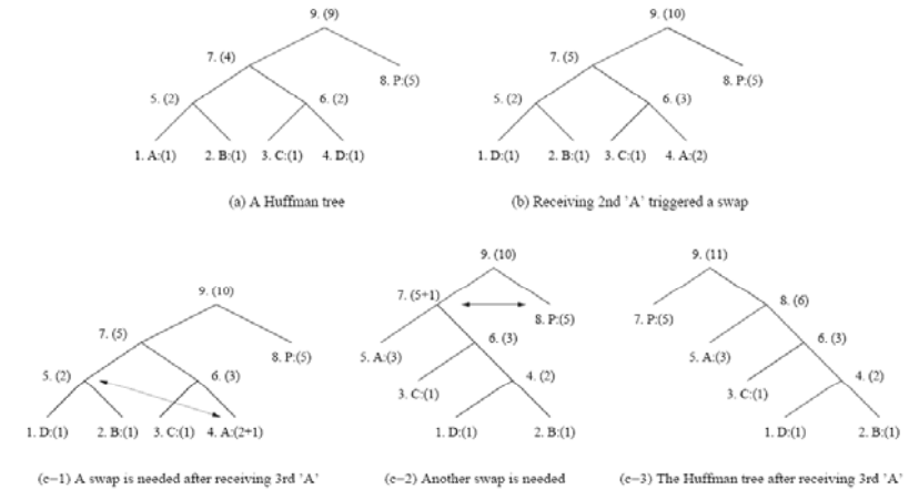
Fig. 7.6: Node Swapping for Updating an Adaptive Huffman Tree
