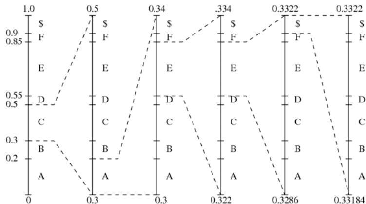
Fig. 7.8(b) Graphical display of shrinking ranges.
