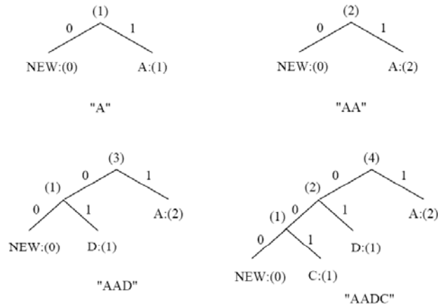
Fig. 7.7 Adaptive Huffman tree for AADCCDD.
