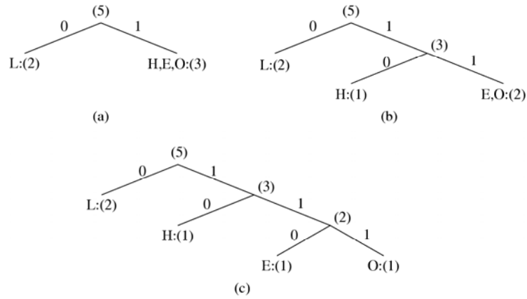
Fig. 7.3: Coding Tree for HELLO by Shannon-Fano.
