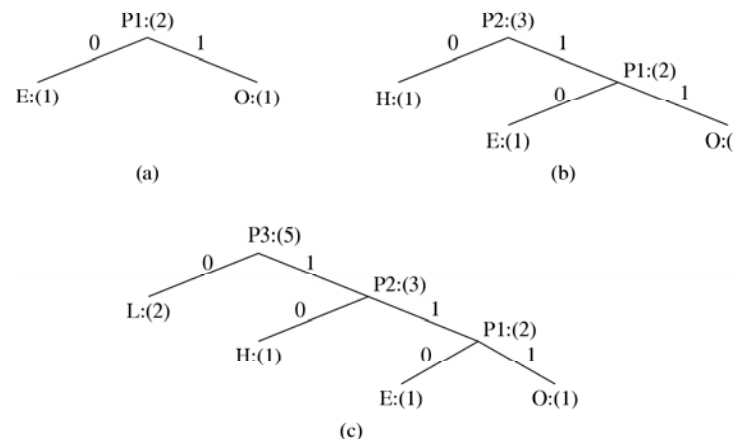
Fig. 7.5: Coding Tree for “HELLO” using the Huffman Algorithm.
