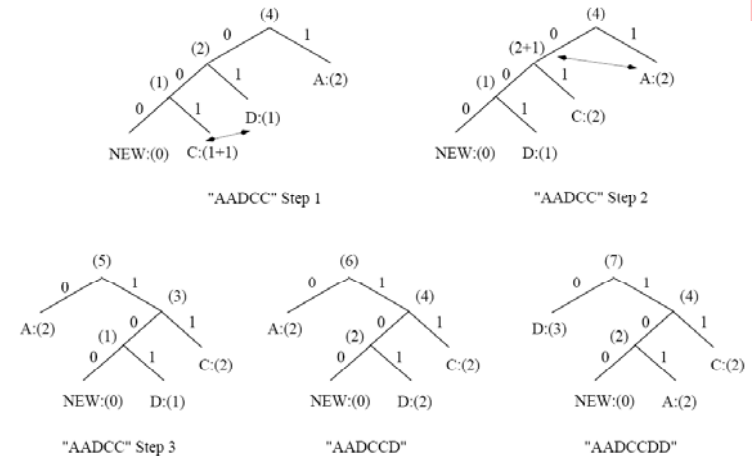
Fig. 7.7 (cont'd) Adaptive Huffman tree for AADCCDD.
